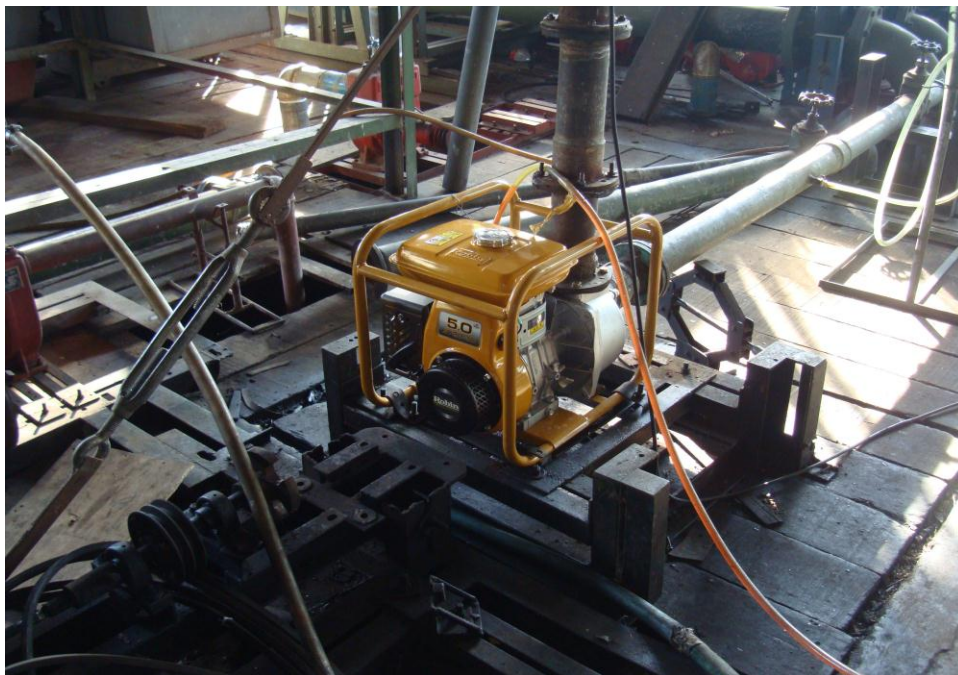
Figure 1. ROBIN PTG305 Pumpset on the test set-up
