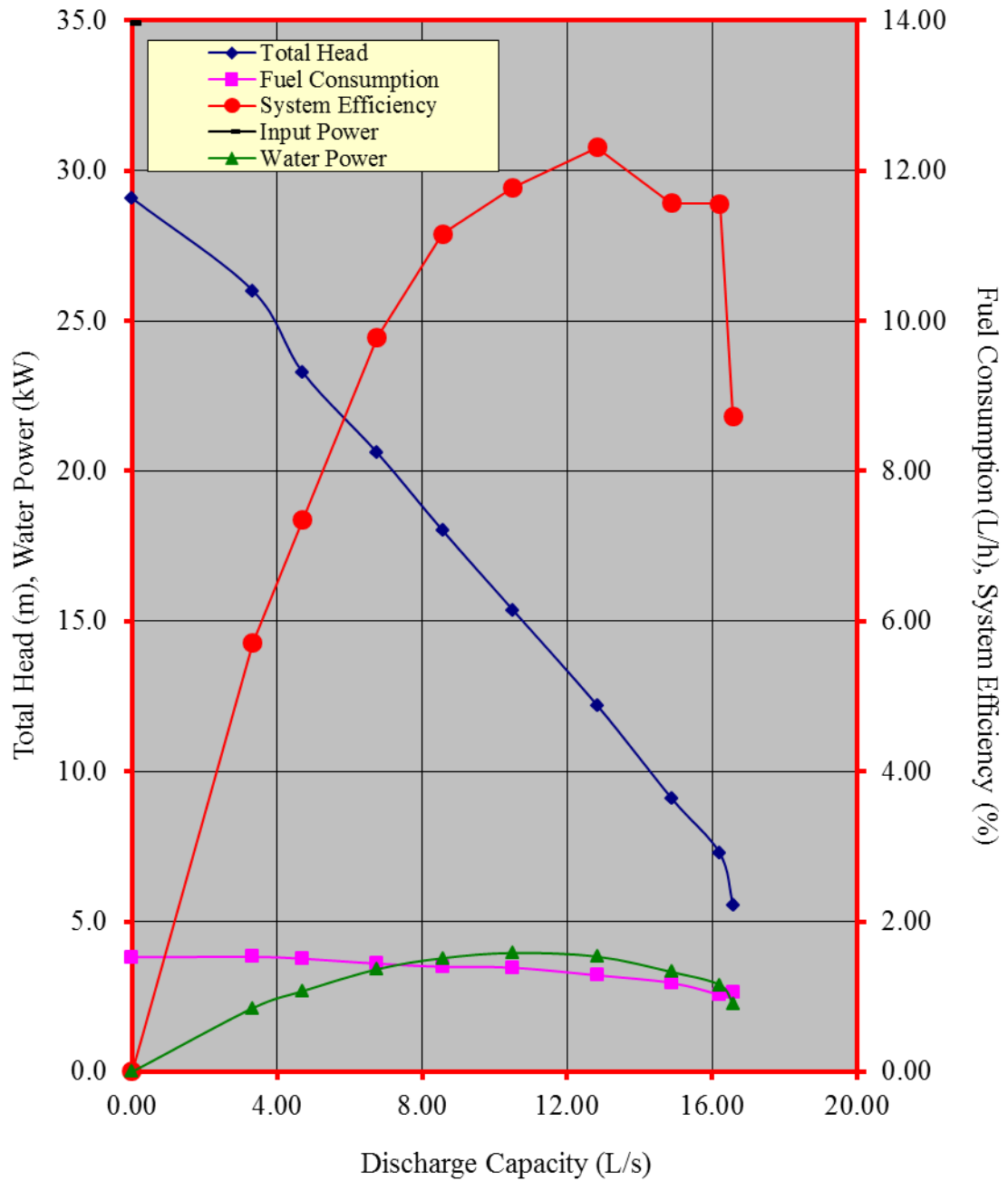
Figure 2. Performance characteristic curves of the ROBIN PTG305 self-priming centrifugal pumpset
